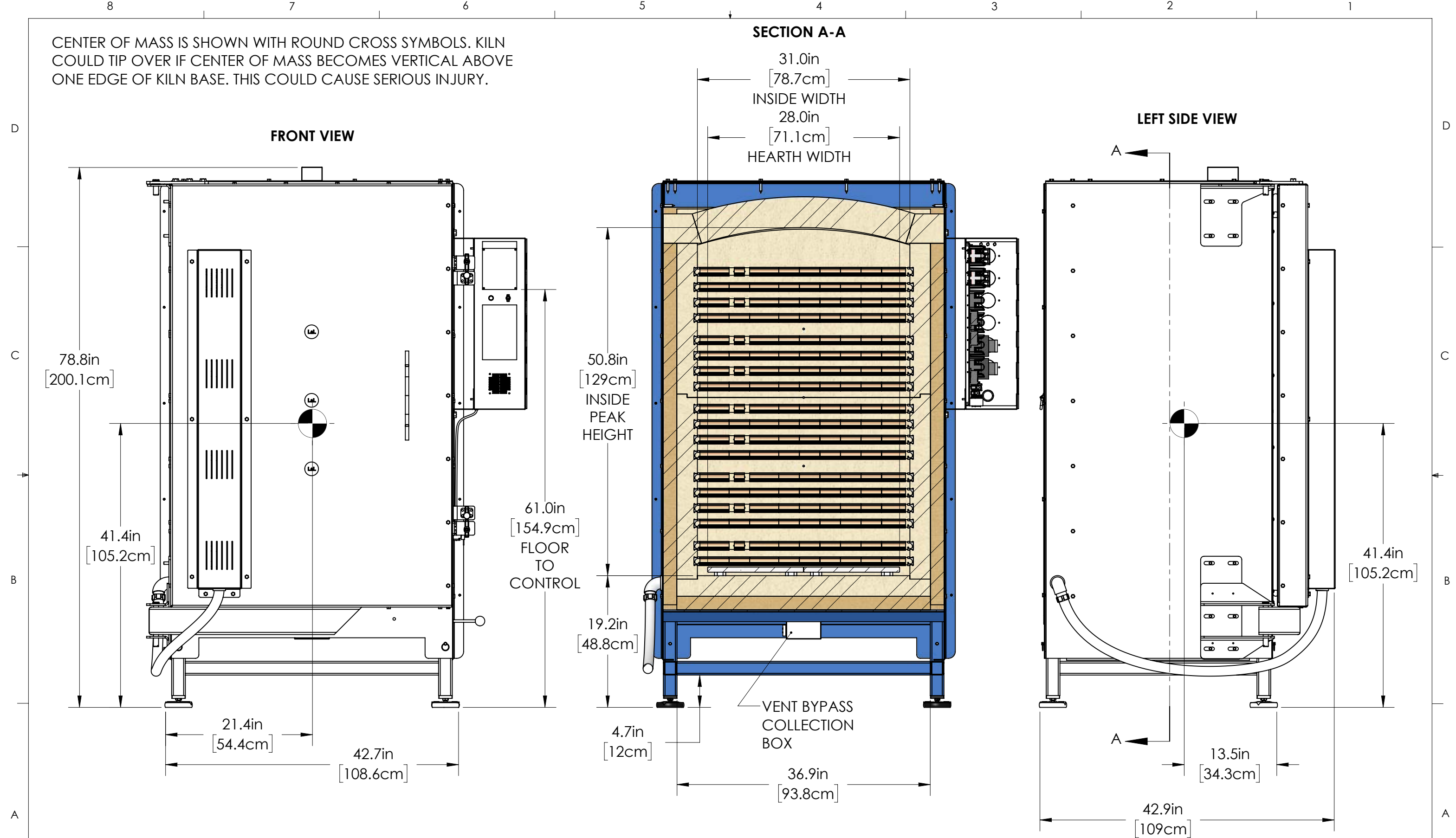
FRONT, FRONT CROSSECTION & LEFT SIDE VIEWS
