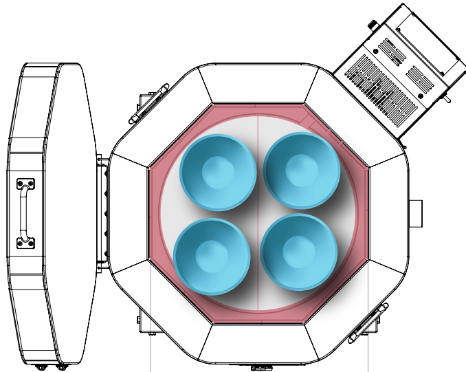
EASY-FIRE e18M-3 TOP VIEW
